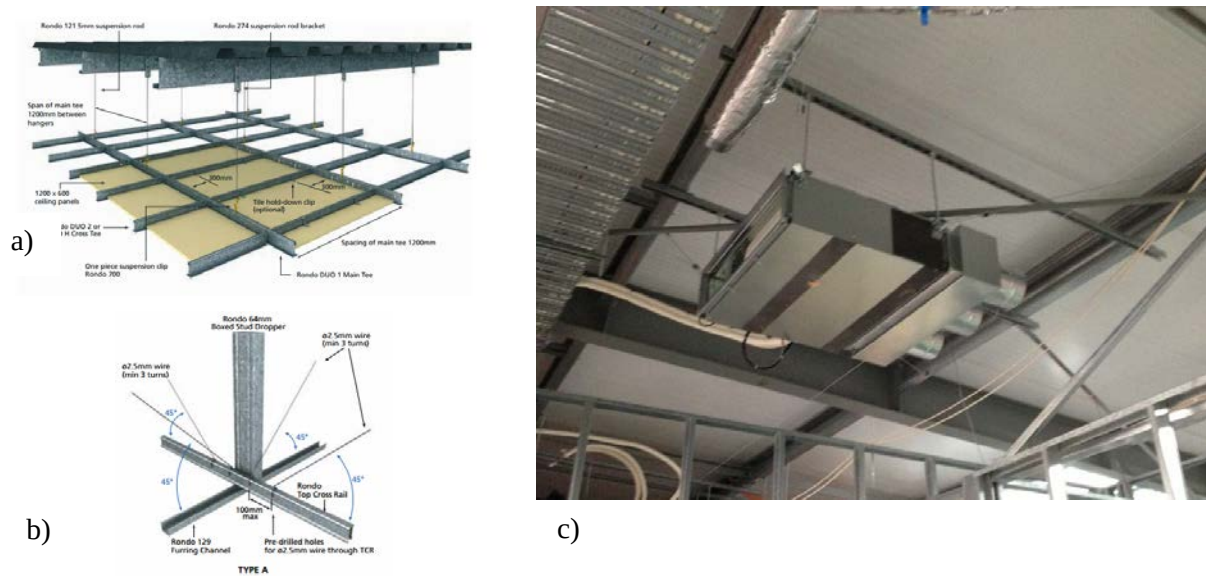
Figure 1. Typical overhead NSE details for: a) Rondo system typical construction, b) typical ceiling bracing, c) typical HVAC unit installation.
